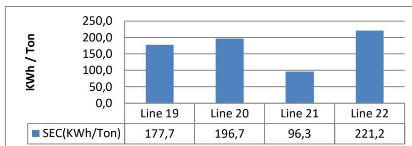
Fig. 3. Specific energy consumption for each production line
