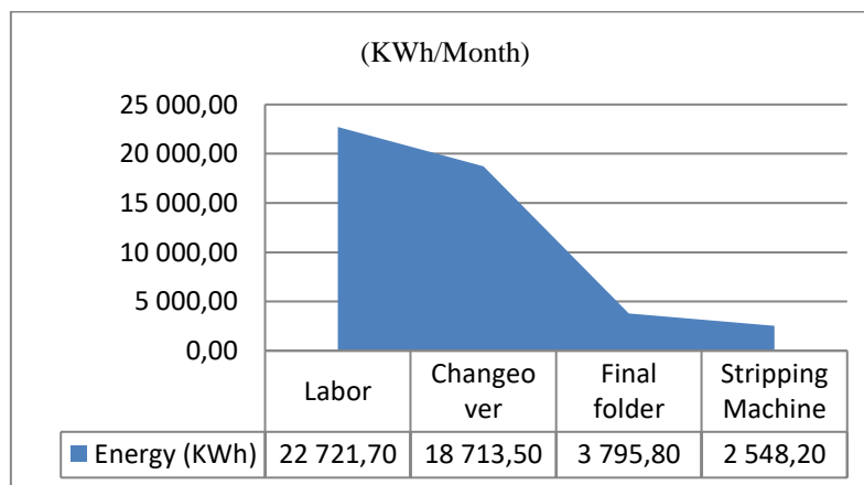
Fig. 6. Energy consumed for the main types of waste in the line 22
