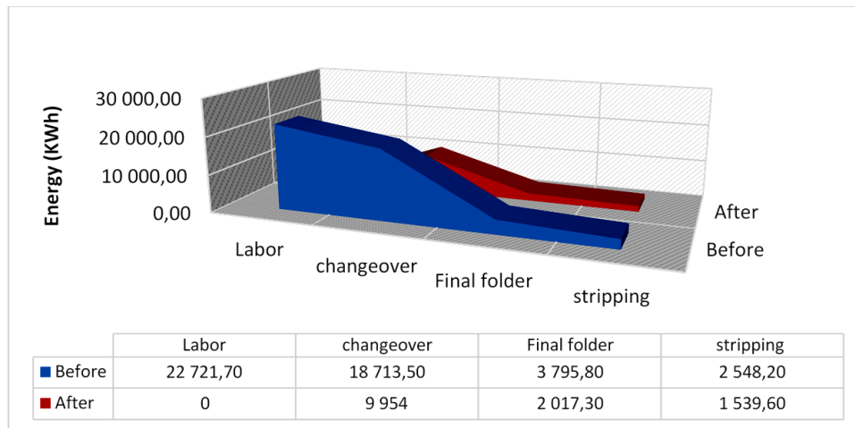
Fig. 11. Change of wasted energy before and after improvement (KWh/Month)
