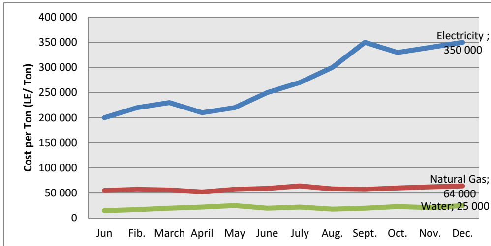
Fig. 2. Different Energy Costs per ton of production
