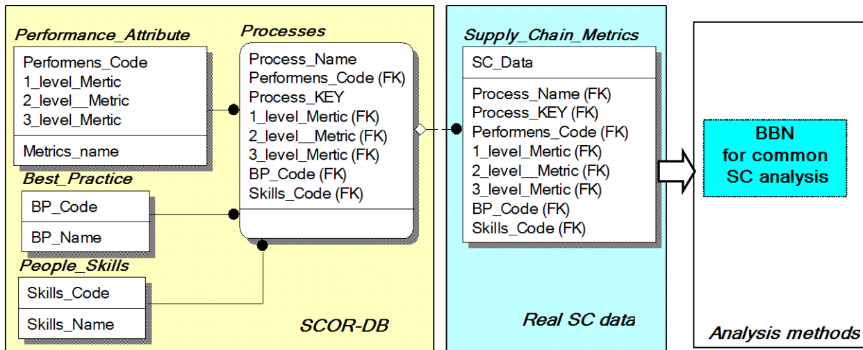
Fig. 2. SCOR-DB structure
