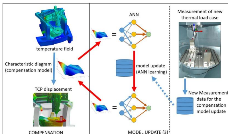
Fig. 2. MRA model updates via ANN training
