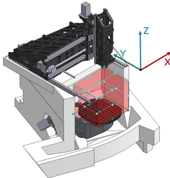
Fig. 1. Workspace of the DMU 80 eVo without housing [17]
