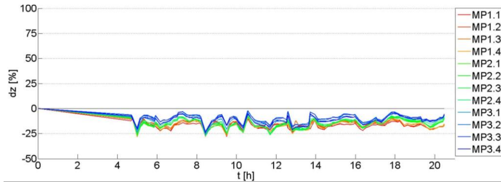
Fig. 7. z-displacement test regime compensated including update
