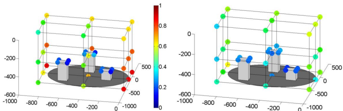
Fig. 3. Workspace support points and measured points (with colour-coded values), left: original values, right: values after all points have been fitted with characteristic diagram
