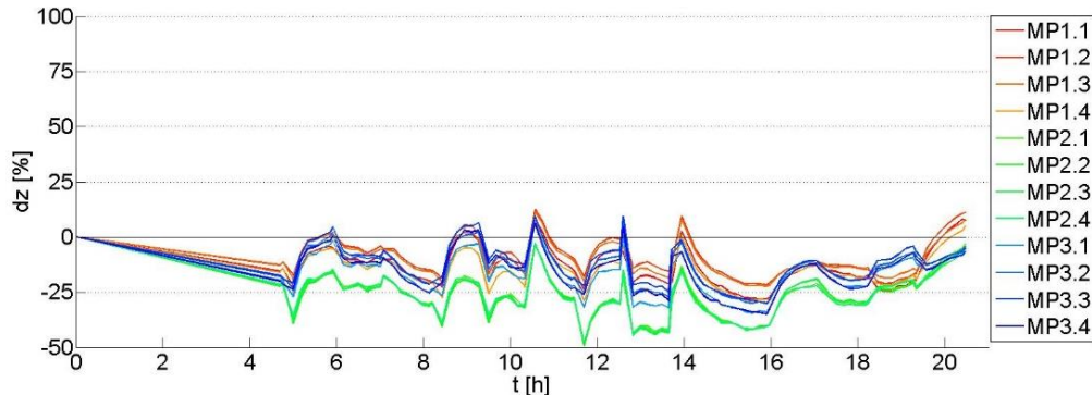
Fig. 6. z-displacement test regime compensated
