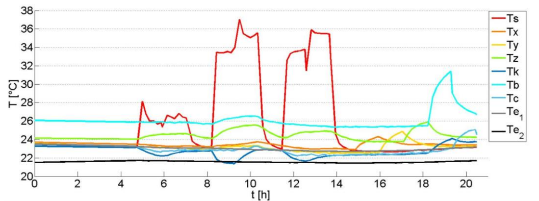
Fig. 4. Temperatures of the test regime (Ts: spindle, Tx: x-axis, Ty: y-axis, Tz: z-axis, Tk: table console, Tb: table b-axis, Tc: table c-axis, Te 1 /e 2 : ambient sensors near the back of the DMU)
