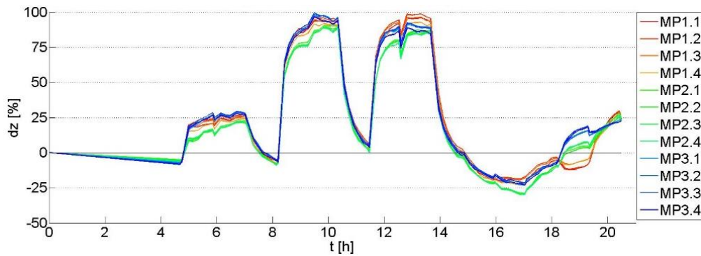
Fig. 5. z-displacement test regime uncompensated
