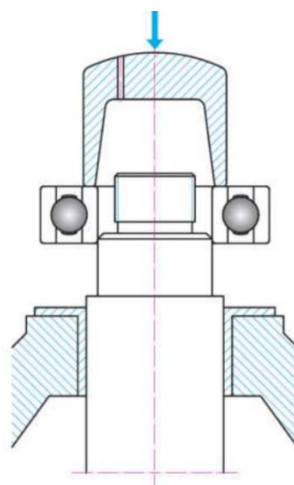
Fig. 2. An example of small bearing assembly [35]
