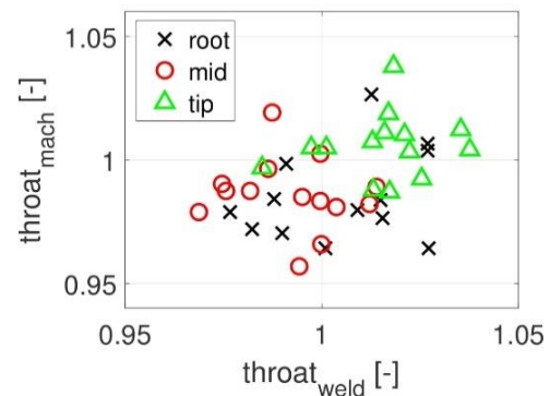
Fig. 17. Correlation of the throat size after welding and after machining
