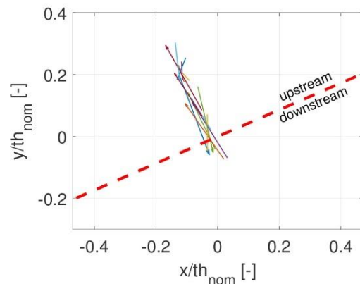
Fig. 19. Vector plot of blade throat centre position change between the production steps at the blade mid-span: (- - -) position of nominal throat
