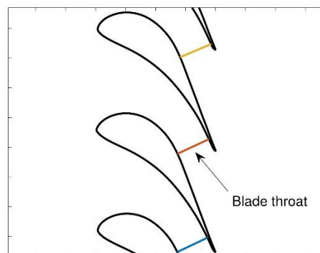
Fig. 5. Unrolled cylinder cross-section of diaphragm blade profiles at the blade mid-span with identified throats, after machining
