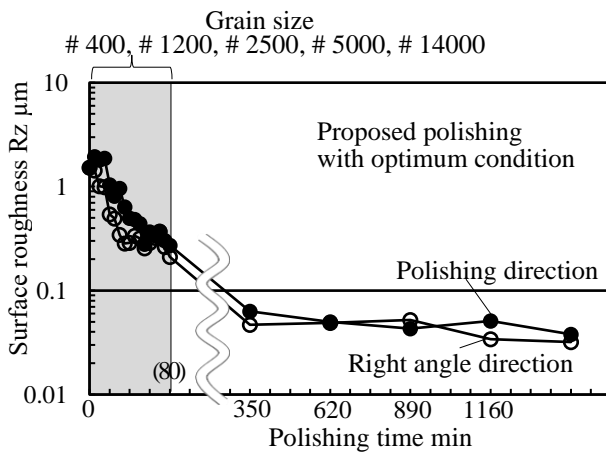
Fig. 8. Relationship between the polishing time and the surface roughness on the workpiece in the polishing process with optimum condition for Titanium. Final surface roughness was Rz\ 0.033\sim 0.038\ \mu\text{m} .
