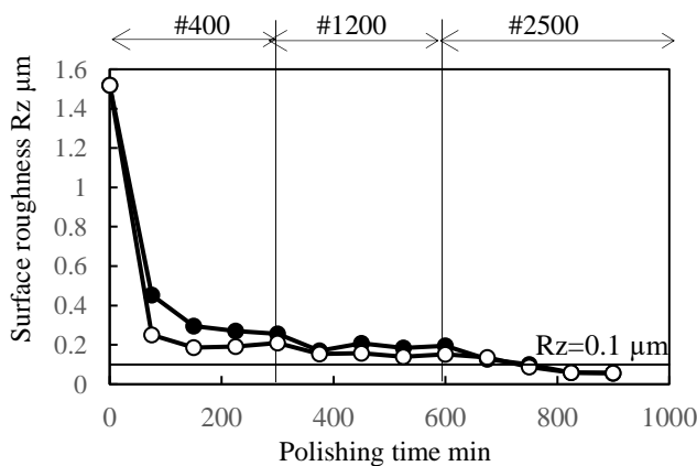
Fig. 4. Relationship between the polishing time and the surface roughness on the workpiece in the polishing process with optimum condition for SUS304. Final surface roughness was Rz 0.05~0.06 μm
