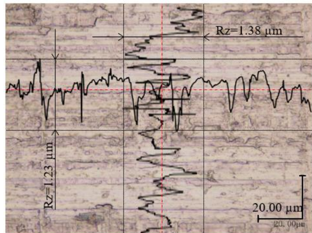
Fig. 7. Photograph on the workpiece (Titanium) after mirror-like polishing using the previous research. Used diamond grain is #50000 after Fig. 6. Surface roughness on the workpiece after mirror-like polishing using the diamond grains #50000. Because the polishing head has contact to the workpiece, surface shape of the polishing head has influence for surface roughness on the workpiece
