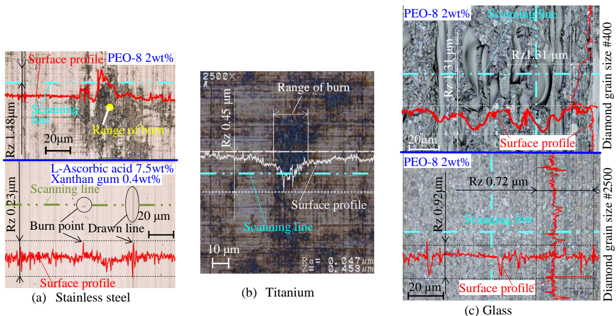
Fig. 2. Photographs on each workpiece with a few faults after polishing process for three medical product materials; stainless steel, titanium and glass. These materials need the several countermeasures to remove the faults
