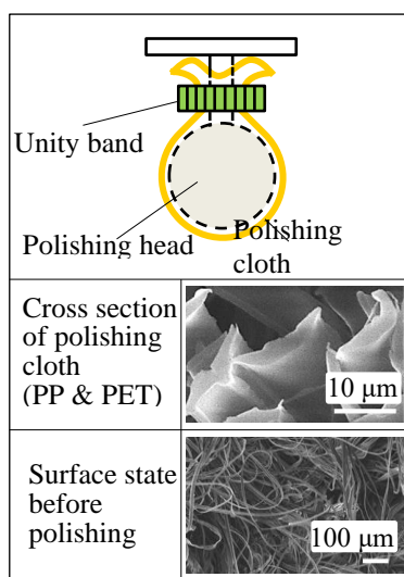
Fig. 3. The improved polishing tool with the nonwoven fabric for mirror-like polishing
