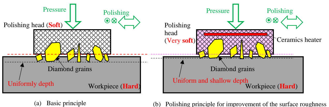
Fig. 1. Schematic view of polishing principle (When the soft tool presses on the hard workpiece, differences between depths of several diamond grains in the workpiece become uniformly)
