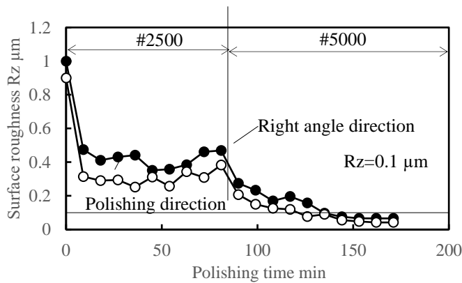
Fig. 10. Relationship between the polishing time and the surface roughness in the polishing process with optimum condition regarding quartz glass
