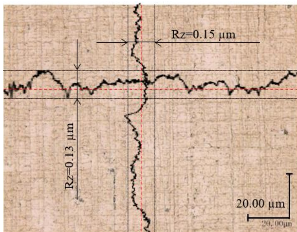
Fig. 6. Photograph on the workpiece (Titanium) after mirror-like polishing using the previous research. Used diamond grains are #400, #1200, #2500, #5000, #14000. Surface roughness on the polishing direction is Rz = 0.13 \mu\text{m} , however, surface roughness on the right angle direction is Rz = 0.147 \mu\text{m} because of the influence of the several polishing draw lines
