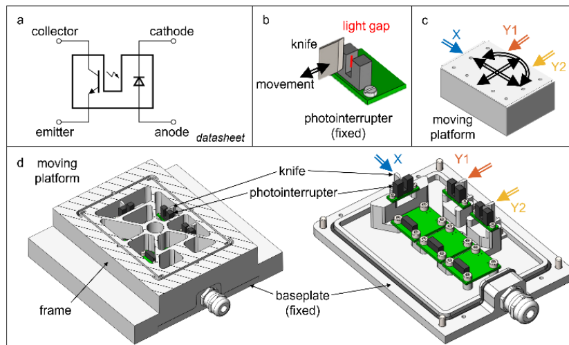
Fig. 3. Knife edge sensors used in the dynamometer
