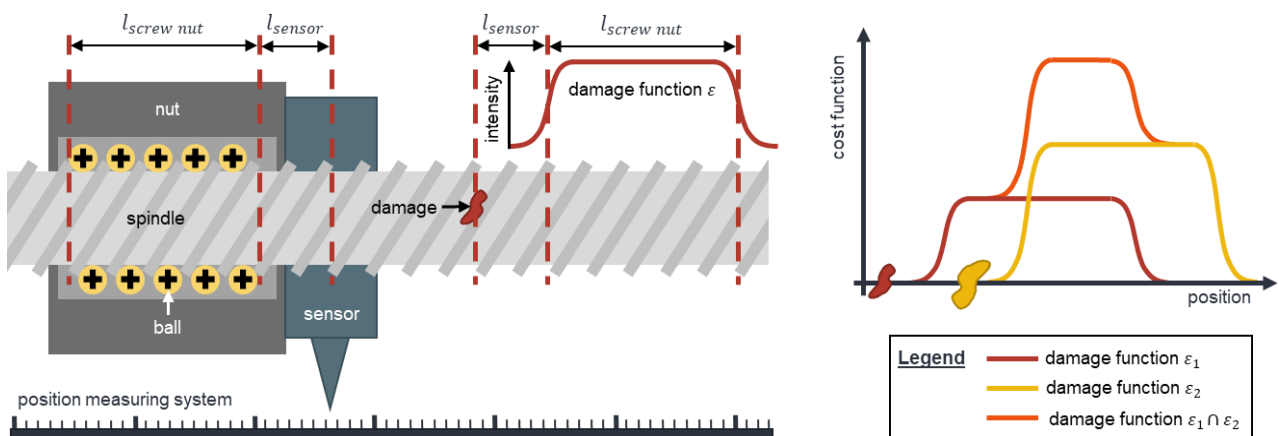
Fig. 3. Optical measuring system attached to the nut of the ball screw drive with the corresponding dimensions (left) as well as the individual and combined damage functions (right)
