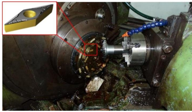
Fig. 2. The cutting Inserts in the Gleason cutting head (gear milling machine 525)
