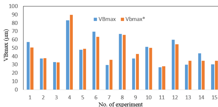
Fig. 9. Measured tool wear (VBmax) and predicted tool wear (VBmax*)
