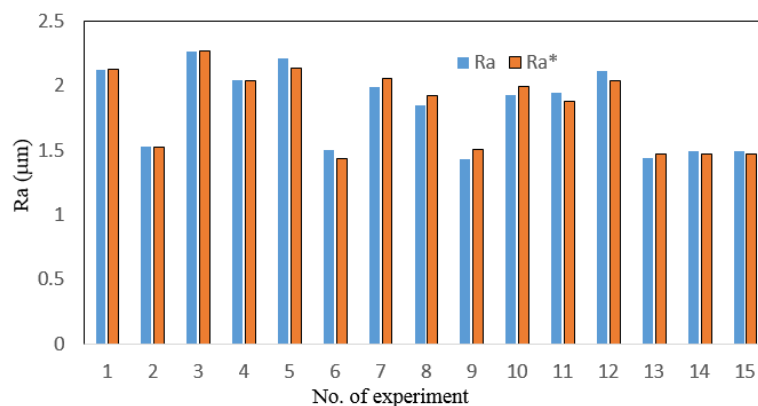
Fig. 8. Measured surface roughness (Ra) and predicted surface roughness (Ra*)
