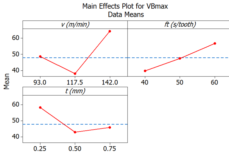
Fig. 7. Influence of cutting parameters on the tool wear
