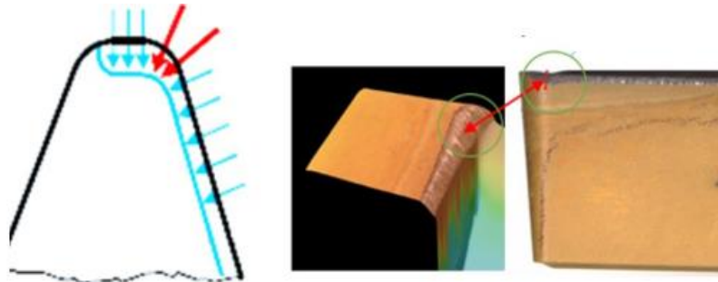
Fig. 5. Measurement position of tool wear
