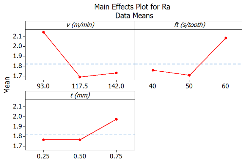
Fig. 6. Influence of cutting parameters on the surface roughness
