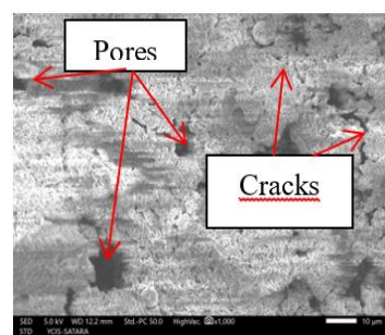
Fig. 14. Cracks on machined surface
