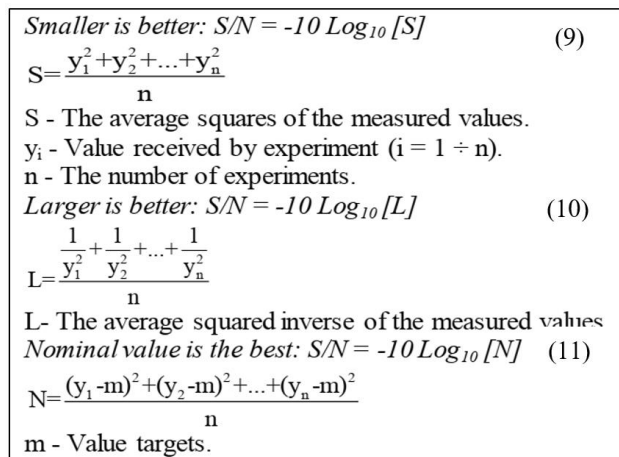
Fig. 7. Determine the value of Signal-to-noise (S/N) ratio
