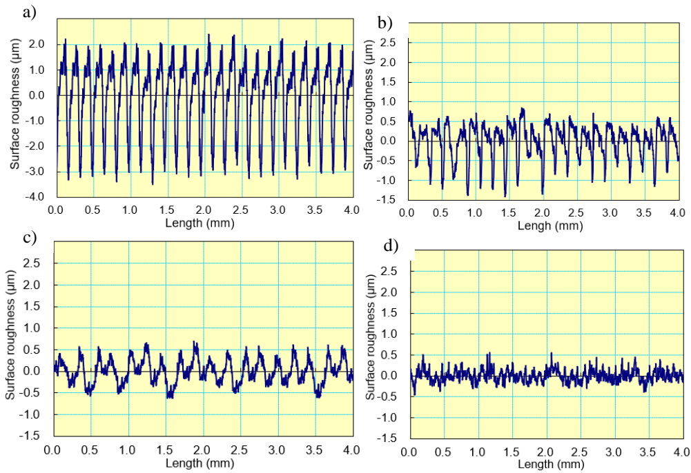
Fig. 5. Surface roughness profile when machining at room temperature (a), 200°C (b), 350°C (c), and 500°C (d)
