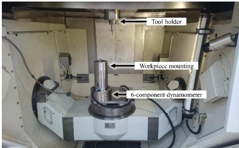
Fig. 3. Experimental setup within the milling machining center LPZ 900 from MAP Werkzeugmaschinen GmbH, Magdeburg, Germany
