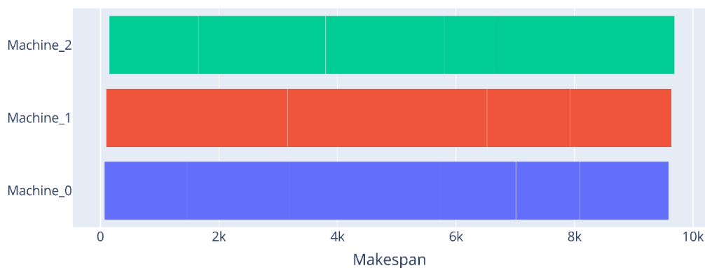
Fig. 1. 17 jobs scheduled on three machines
