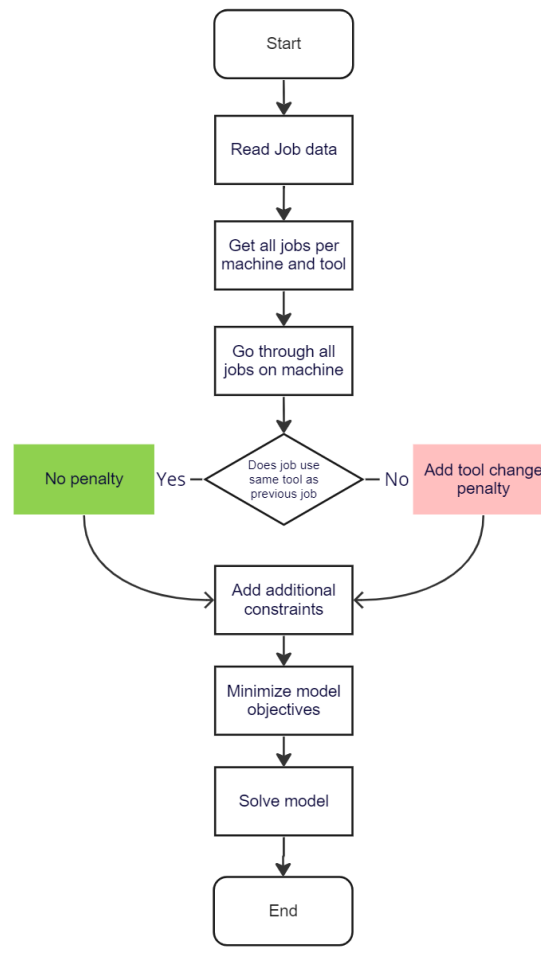
Fig. 2. Flow Diagram of the job allocation algorithm and tool change penalty
