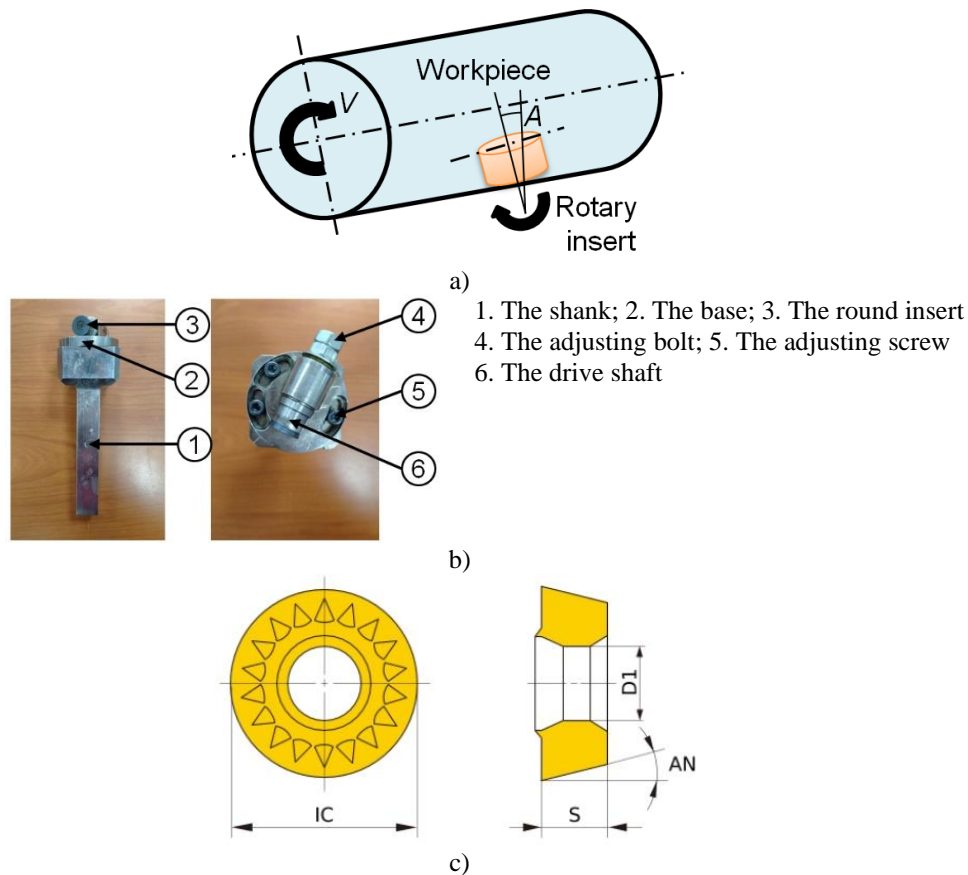
Fig. 1. The concept of the HRT process: a) – the schematic principle, b) – the fabricated rotary tool, c) – the round insert
