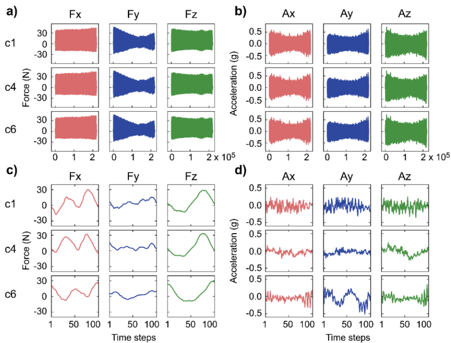
Fig. 3. Raw data of forces ( F_x , F_y , and F_z ) and vibration accelerations ( A_x , A_y , and A_z ) for a single cut (top) and 100 time step windows (bottom). The data is presented for cut number 150
