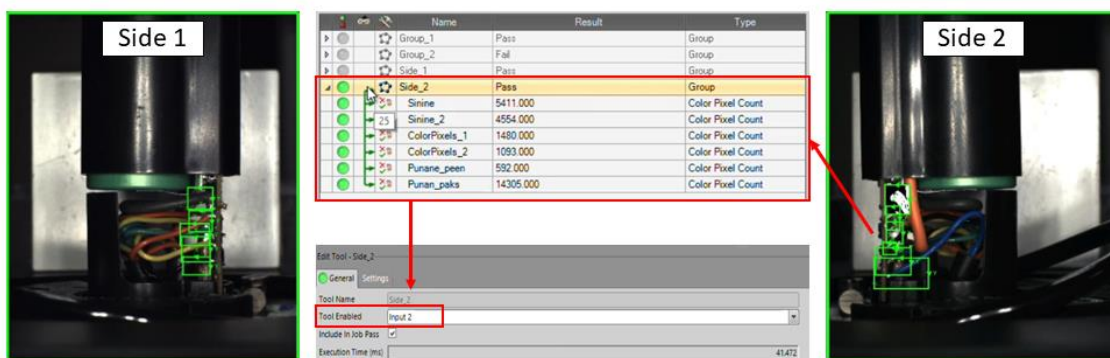
Fig. 2. An example of MV program structure
