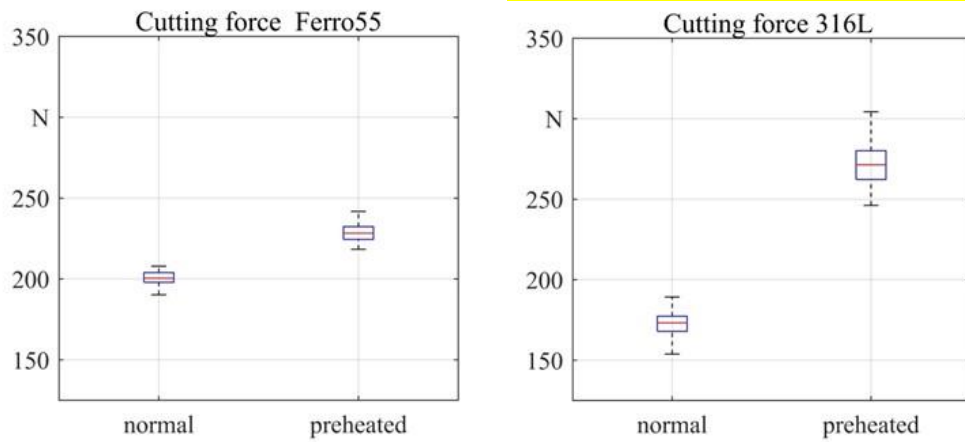
Figure 9. Cutting forces of Ferro55 and 316L samples
