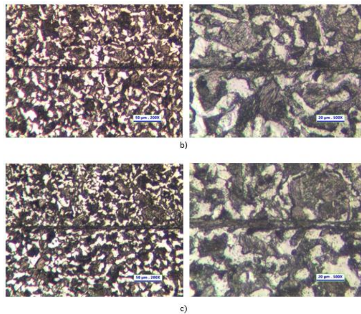
Fig. 13. Interface comparison amongst (a) press-fitting, (b) shrink-fitting, and (c) ultrasonic oscillated shrink-fitting
