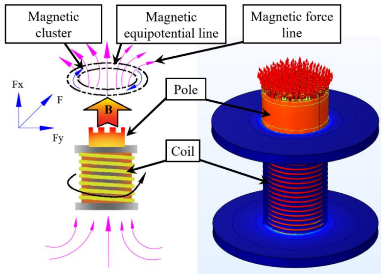
Fig. 1. Schematic of the Magnetic Force Elements within a Magnetic Field
