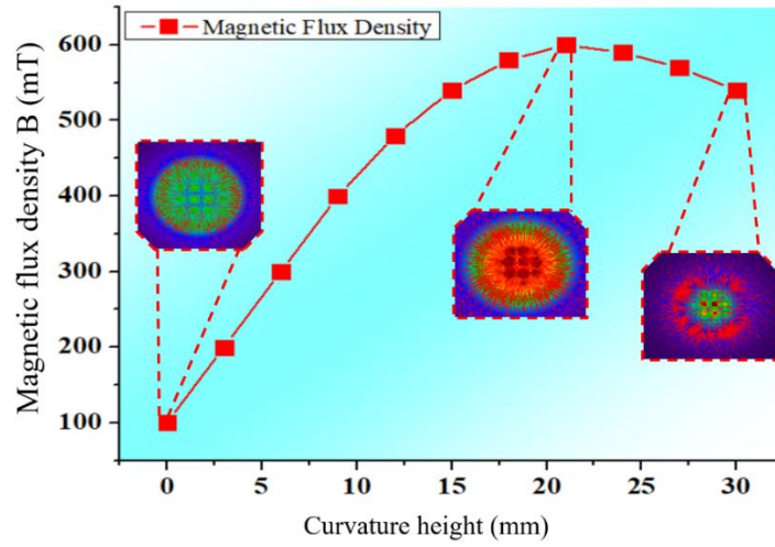
Fig. 6. Optimal Curvature of Convex Pole Tip
