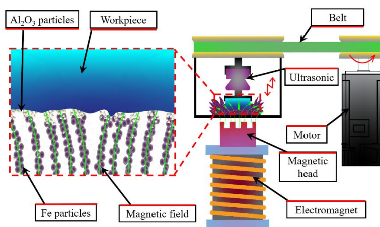
Fig. 2. The ultrasonic-assisted magnetic abrasive finishing (UAMAF)
