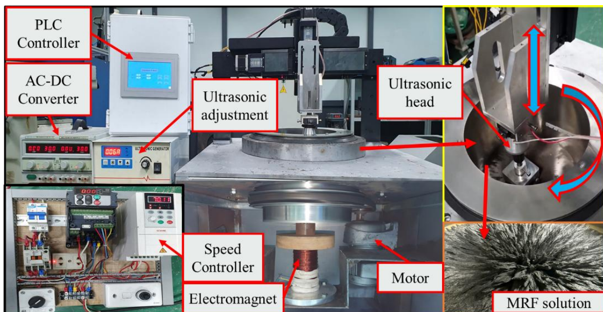
Fig. 7. Experimental setup
