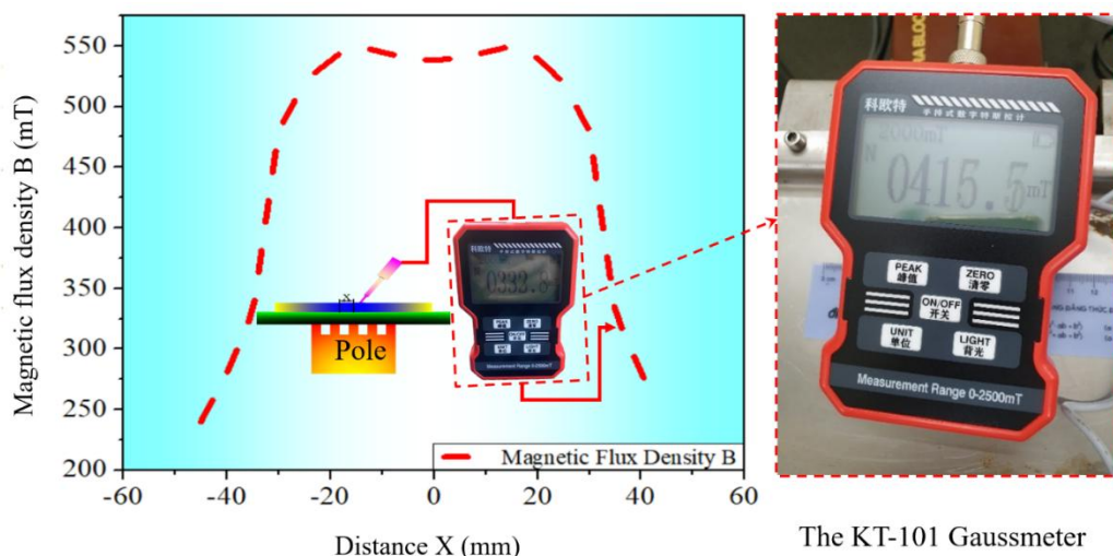
Fig. 3. Experimental setup for magnetic field measurement using the KT-101 Gaussmeter and field visualization system
