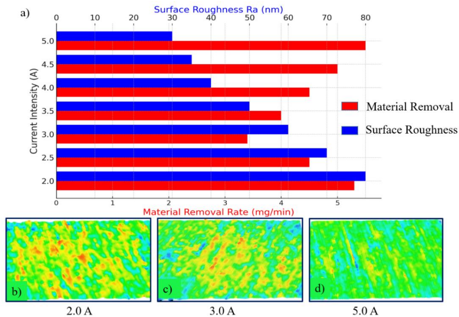
Fig. 9. Electric current affects the ability to remove materials
