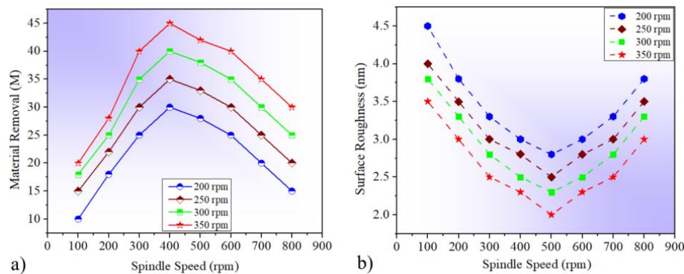
Fig. 8. Effect of Speed on Material Removal Rate: a) Material removal at different spindle speeds; b) Surface roughness at different spindle speeds
