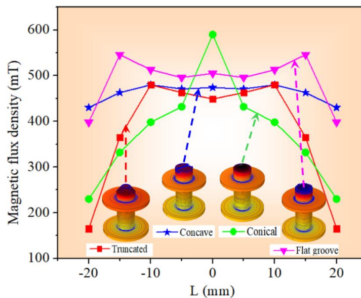
Fig. 4. Magnetic Field Magnitude of the Electromagnets
