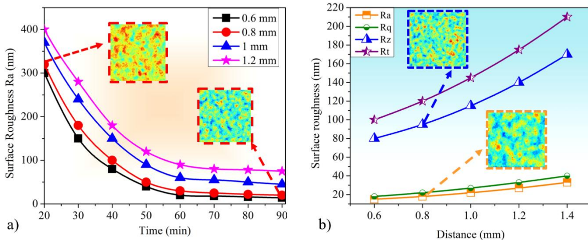
Fig. 10. Effect of polishing distance on surface finish: a) Surface roughness at different polishing distances, b) Surface roughness parameters at different polishing distances
