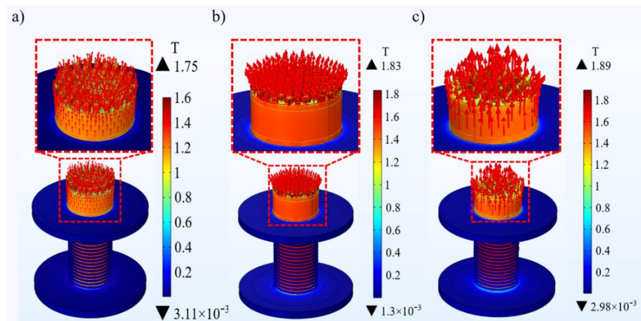
Fig. 5. Magnetic Field Intensity of Different Pole Types: a) Concave, b) Flat, c) Convex
