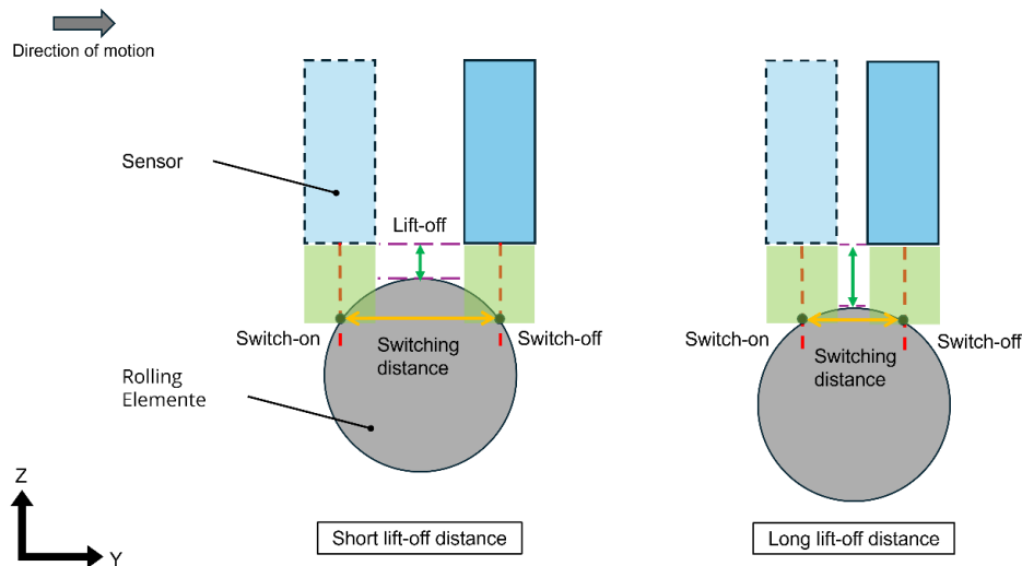
Fig. 2. Concept of the measurement method
