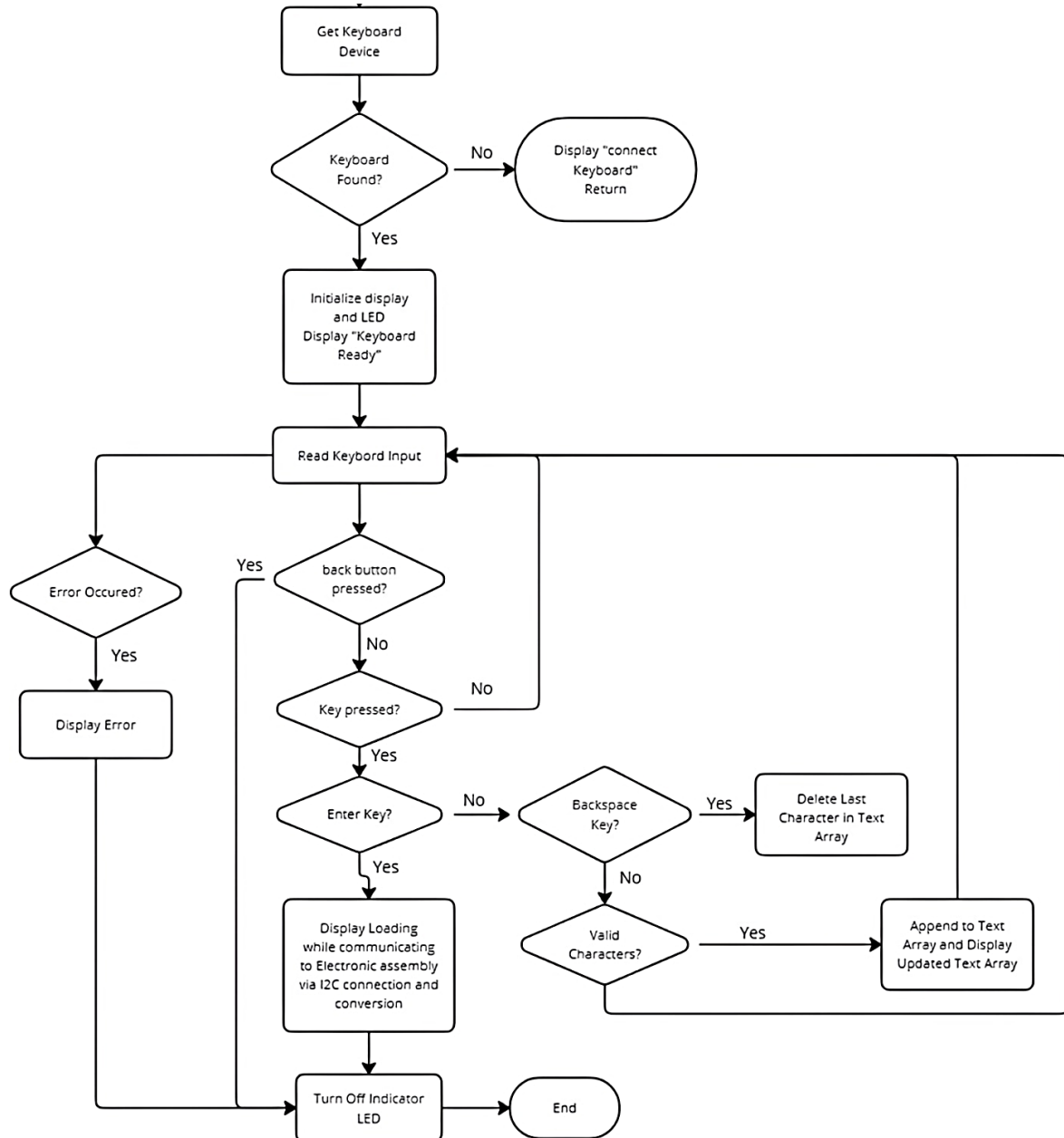
Fig. 4. Keyboard Flow
