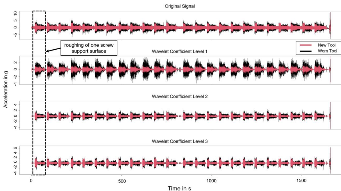
Fig. 3. Wavelet decomposition of acceleration signal of roughing process
