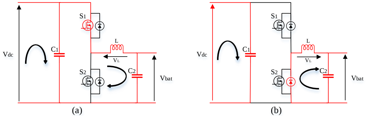
Fig. 4. Buck mode: (a) when S_1 is ON, (b) when S_1 is OFF
