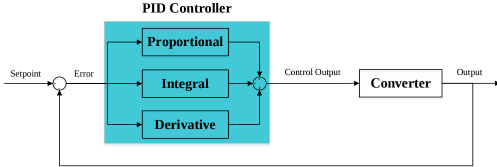
Fig. 6. Block diagram of PID controller
