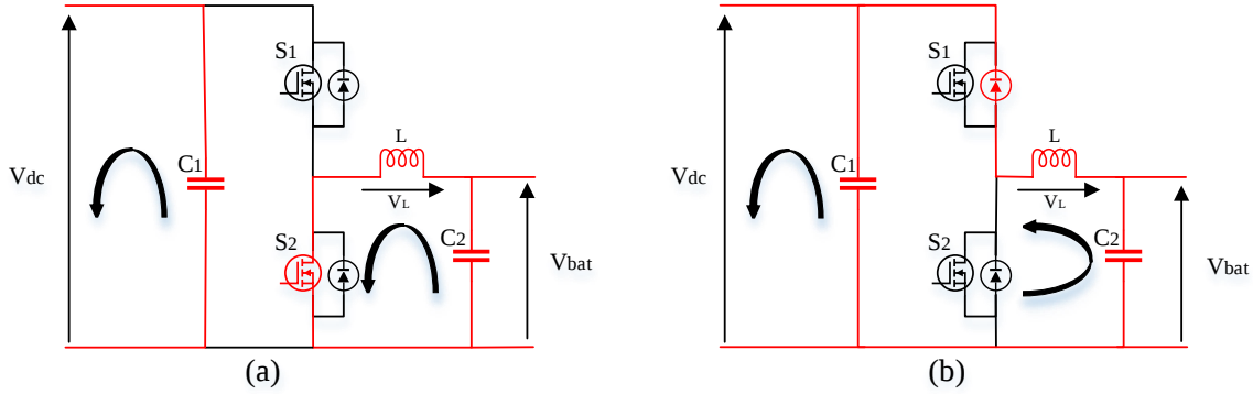
Fig. 5. Boost mode: (a) when S_2 is ON, (b) when S_2 is OFF
