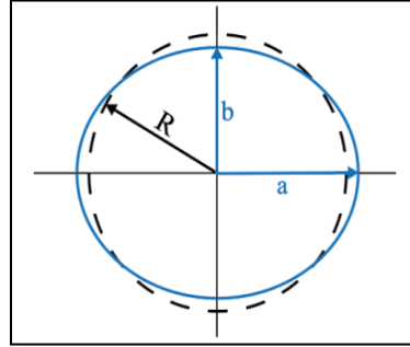
Fig. 4. Elliptical Deviations
