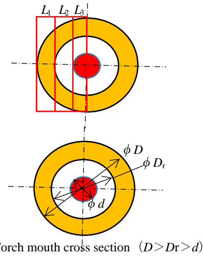
Fig. 14. Specification of the ring torch
