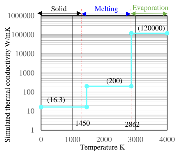
(f) Simulated thermal conductivity D for bottom region
