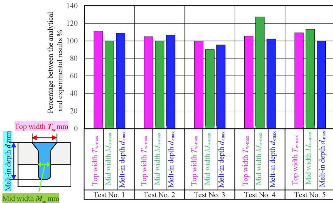
Fig. 20. Percentage of relation between the analytical and experimental results
