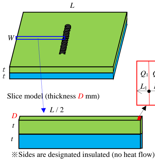
Fig. 13. Heat generation setting for analysis with ring torch
