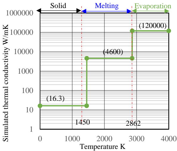
(c) Simulated thermal conductivity A for region directly under the torch
