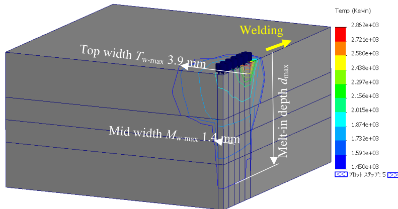
Fig. 18. Temperature distribution at t=0.1615 sec regarding Test No. 4 (Blue line: melting point)
