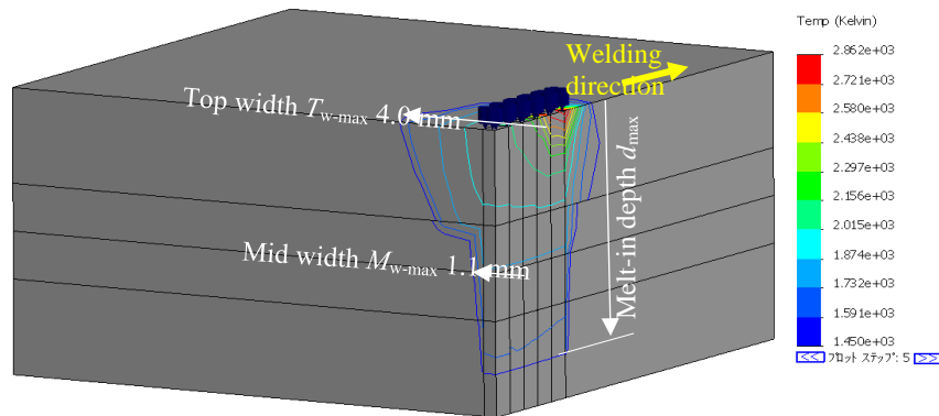
Fig. 15. Temperature distribution at t=0.1615 sec regarding Test No. 1 (Blue line: melting point)
