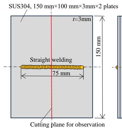
Fig. 3. Schematic view of the evaluation experiment
