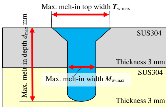
Fig. 2. Definition of quality evaluation factors for laser keyhole welding
