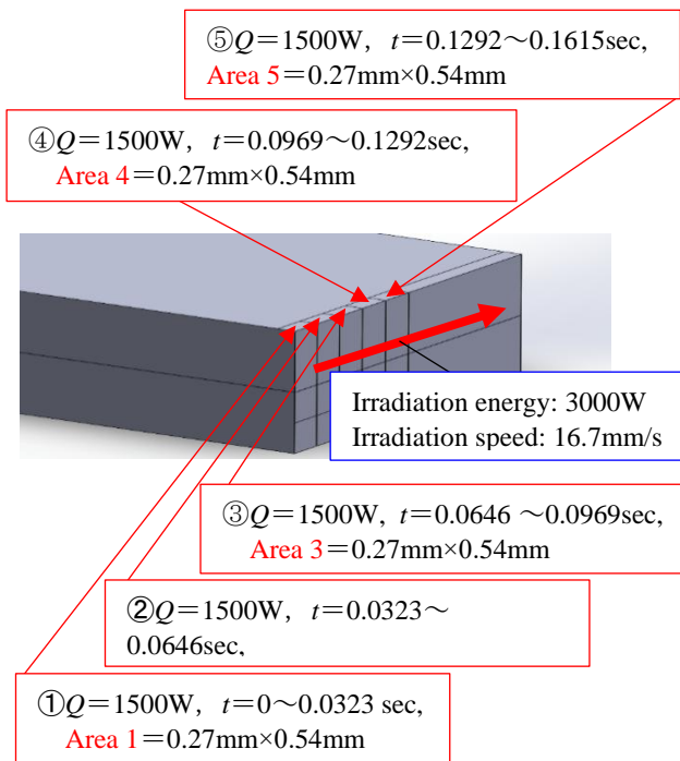
Fig. 11. Relationship between the irradiation energy and each area for the travelling irradiation
