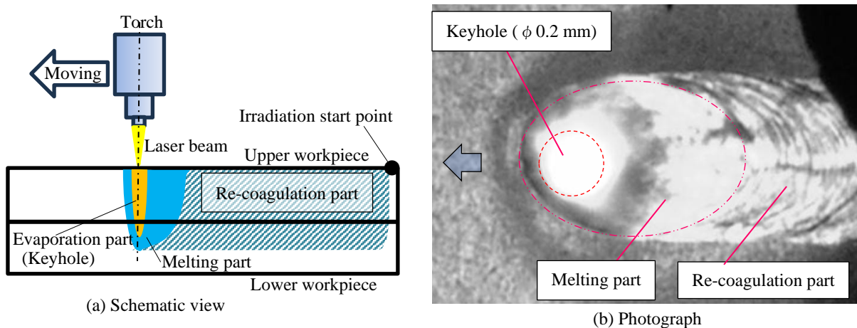
Fig. 1 Schematic view and photograph of the laser keyhole welding
