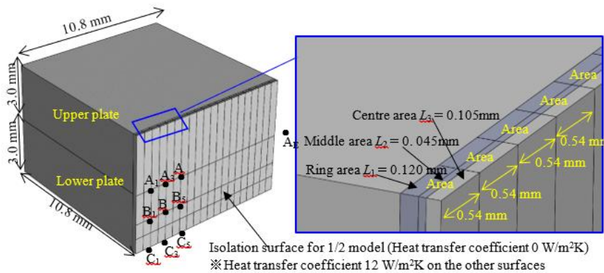
Fig. 9. FEM model for laser keyhole welding of SUS 304 (1/2 model)
