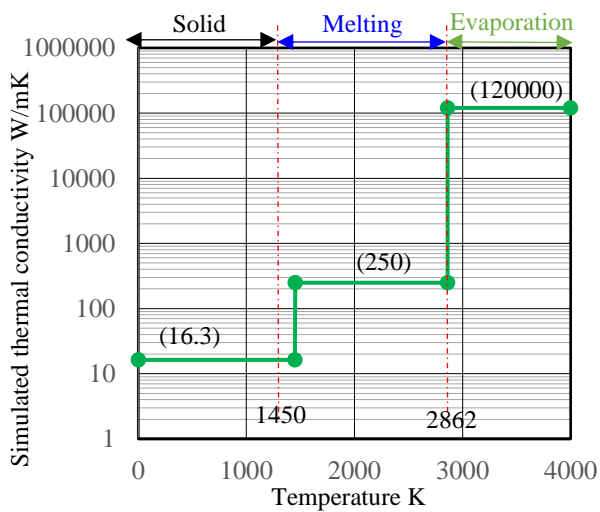
(e) Simulated thermal conductivity C for middle region
