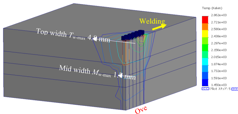
Fig. 19. Temperature distribution at t=0.323 sec regarding Test No. 5
