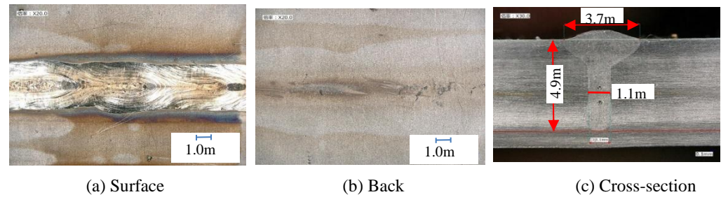
Fig. 7. Photograph after laser welding__Test No. 4
