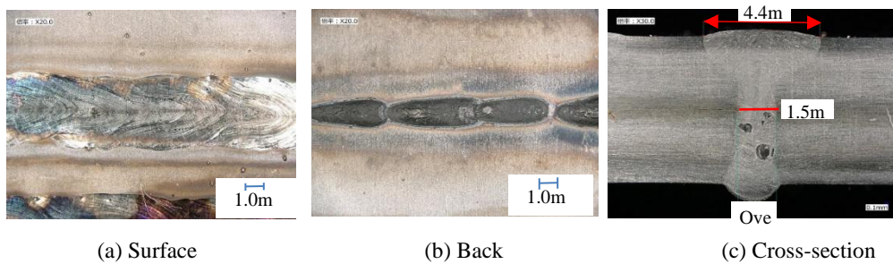
Fig. 8. Photograph after laser welding__Test No. 5
