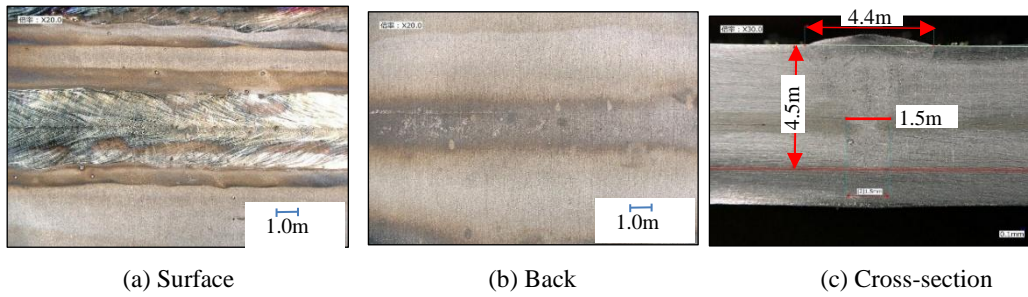
Fig. 5. Photograph after laser welding__Test No. 2
