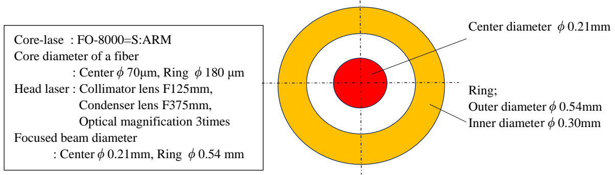
Fig. 12. Specification of the ring type laser torch
