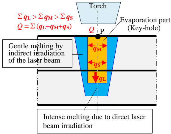
(a) Schematic view of heat inflow from the keyhole to the melt region and the flow state in the melt region at that time
