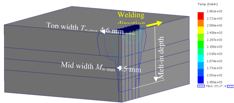
Fig. 16. Temperature distribution at t=0.323 sec regarding Test No. 2 (Blue line: melting point)
