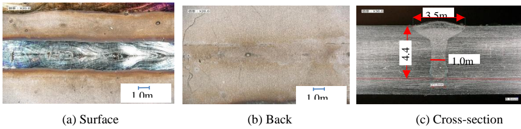
Fig. 6. Photograph after laser welding__Test No. 3
