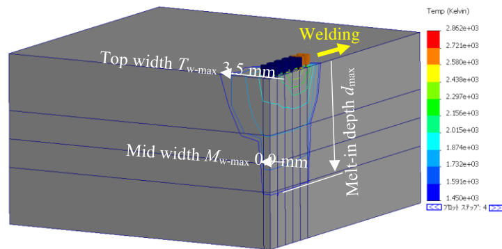
Fig. 17 Temperature distribution at t=0.1615 sec regarding Test No. 3 (Blue line: melting point)
