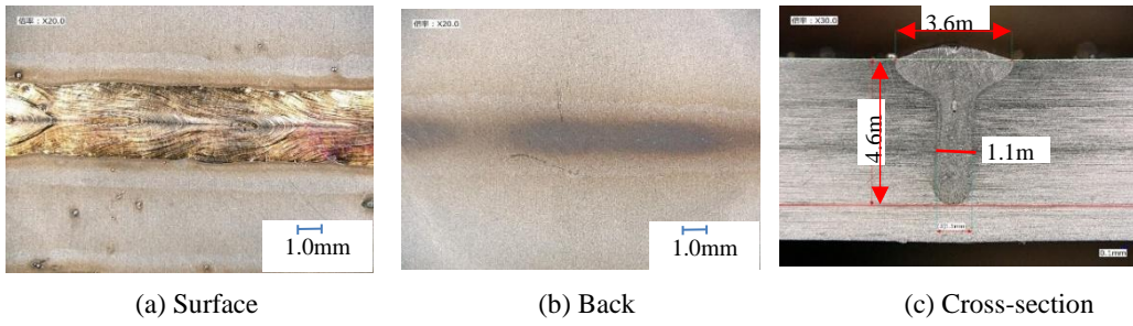
Fig. 4. Photograph after laser welding__Test No. 1
