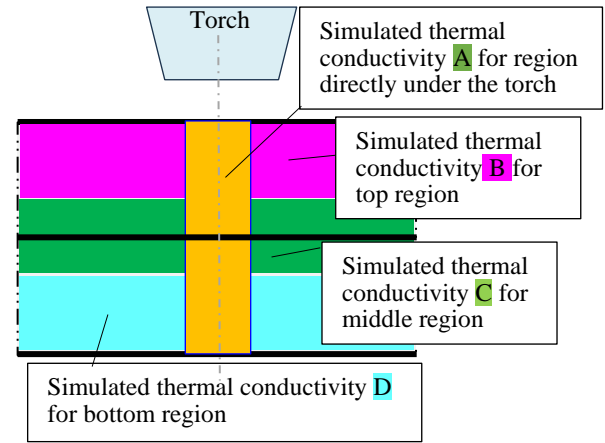
(b) Setting up four thermal conductivity regions taking into account the heat inflow from the keyhole to the melt region
