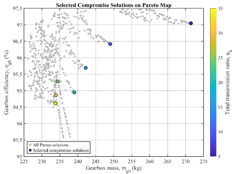
Fig. 8. Selected compromise solutions projected onto the global Pareto map
