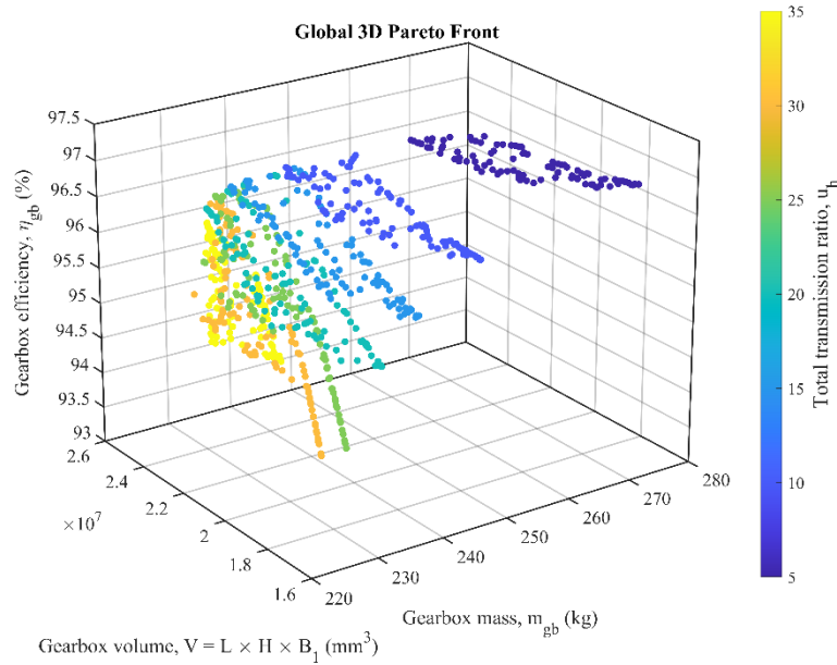
Fig. 7. Global three-dimensional Pareto front considering gearbox mass, gearbox volume, and gearbox efficiency
