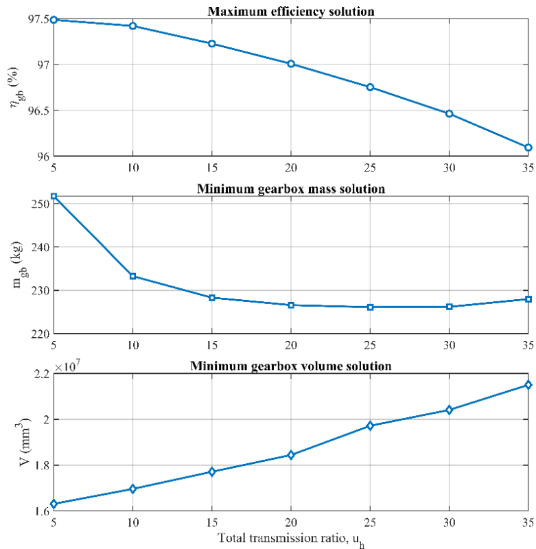
Fig. 4. Effect of the total transmission ratio on the maximum-efficiency solution, minimum-mass solution, and minimum-volume solution
