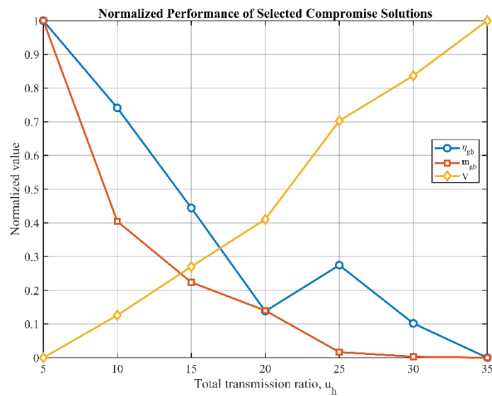
Fig. 10. Normalized performance comparison of the selected compromise solutions
