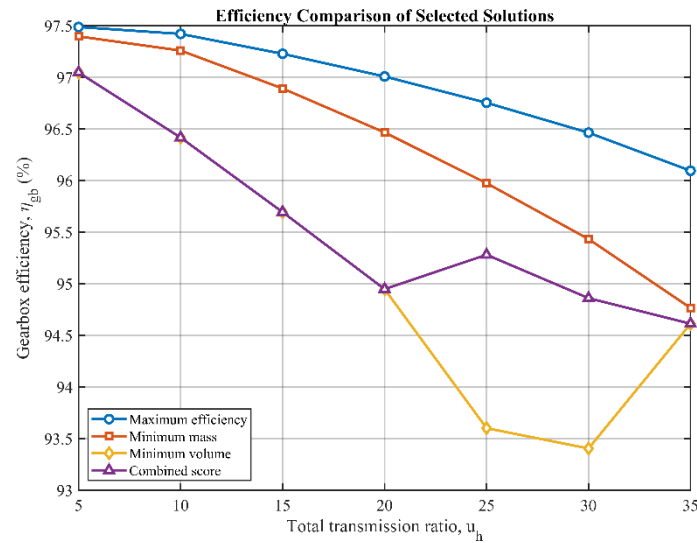
Fig. 5. Efficiency comparison among representative Pareto-optimal solutions
