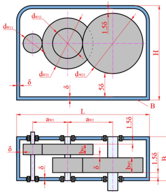
Fig. 1. Scheme for calculation of gearbox mass
