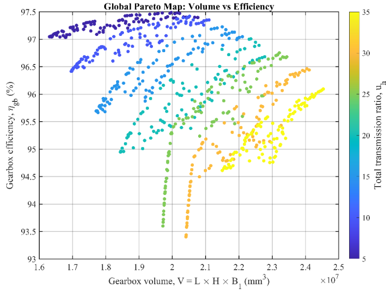
Fig. 3. Global Pareto map showing the relationship between gearbox volume and gearbox efficiency under different transmission ratios
