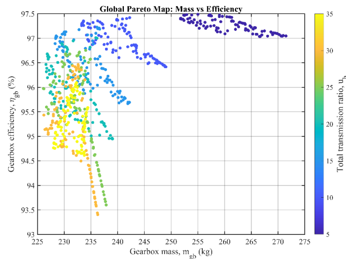
Fig. 2. Global Pareto map showing the relationship between gearbox mass and gearbox efficiency for different total transmission ratios
