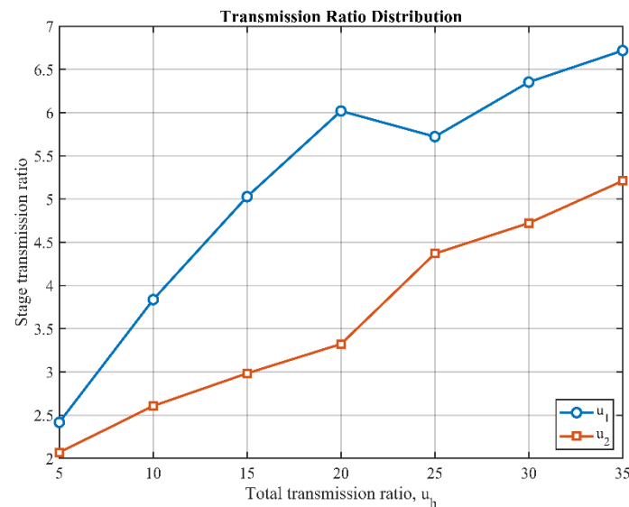
Fig. 6. Distribution of first-stage and second-stage transmission ratios for the selected compromise solutions
